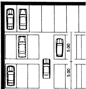
⑥ Private parking, 3 cars stacked vertically
